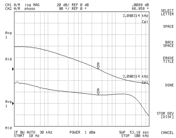
Loop Gain & Phase at V_i=48V , Full Load
