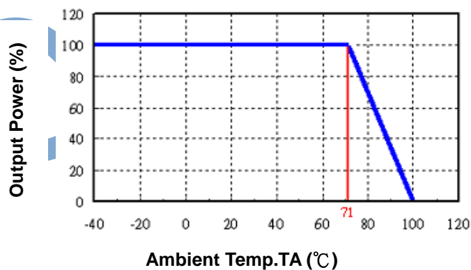
BOB5W Series Power Derating Curve(5)
